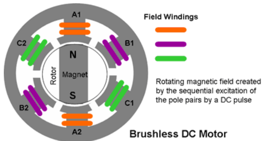
FIGURE 4: BASIC DIAGRAM OF BRUSHLESS DC MOTOR
